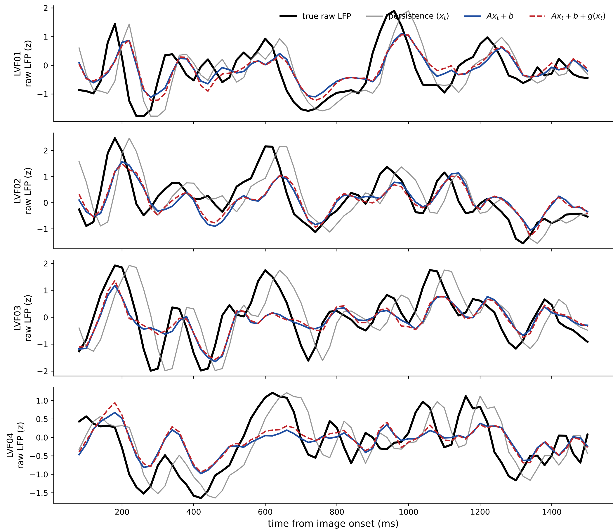
Predictions following the raw LFP — held-out trial 41, \Delta = 40 ms (P12 · LVF · raw broadband)
