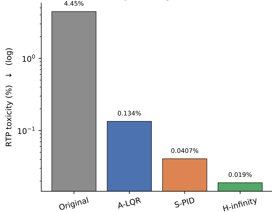
B. Toxicity steering (DistilGPT-2)
