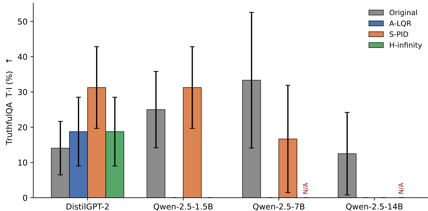
A. Truthfulness across model scales
