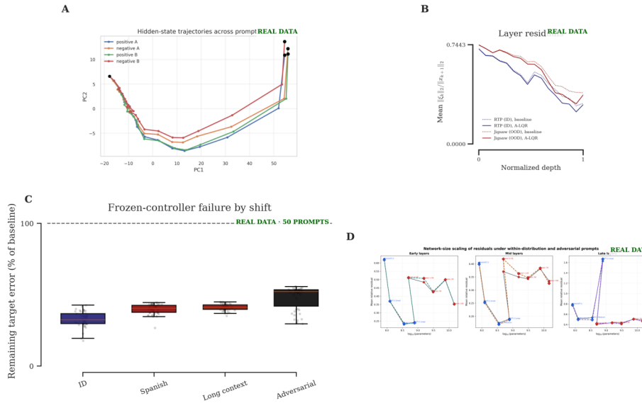
Figure 4 — ID benchmark
