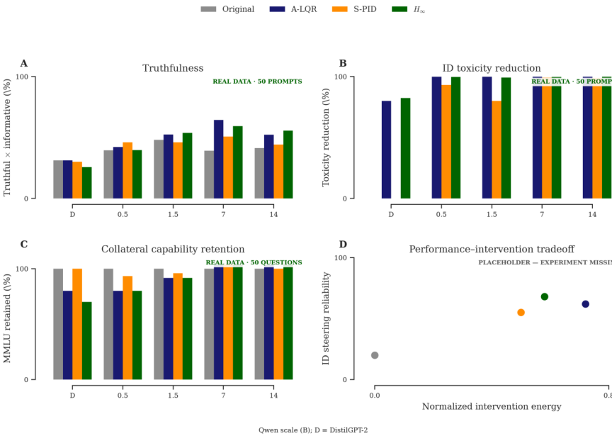
Figure 4 — ID benchmark
