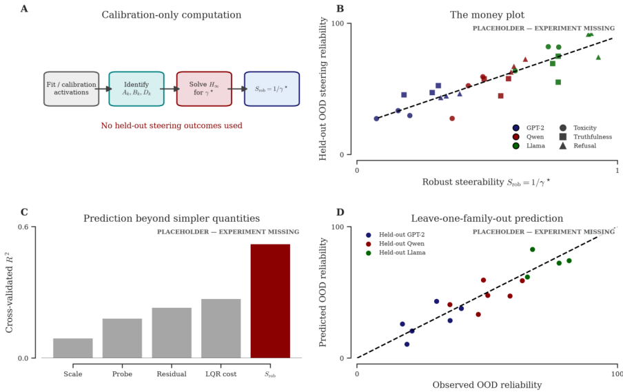
Figure 5 — OOD benchmark
