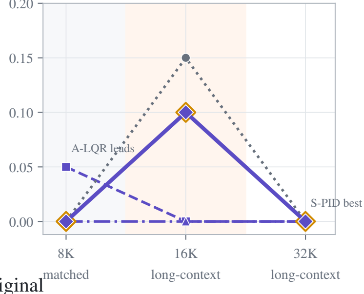
C Overall steering (0-2)
