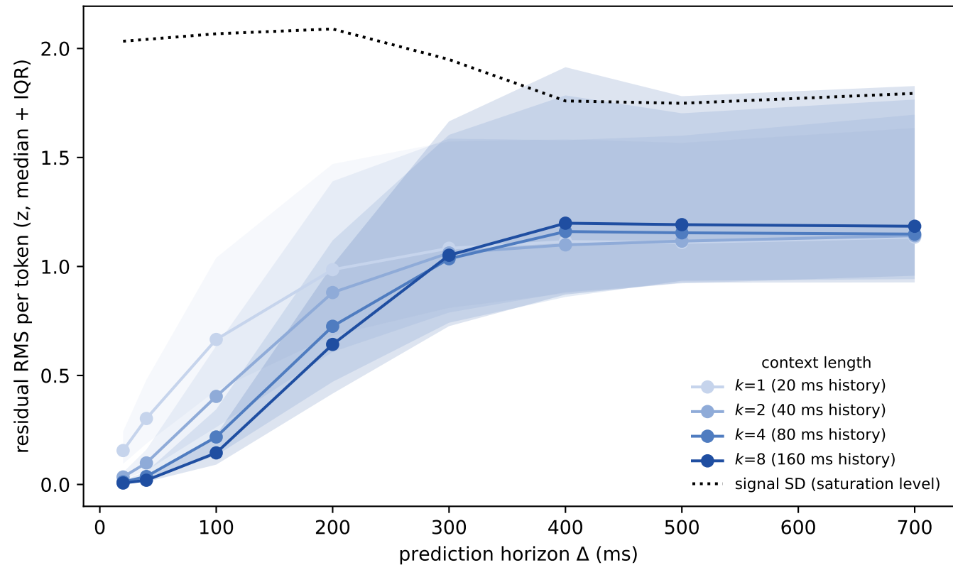
Panel F (residual version) — longer context delays residual growth (P12 · LVF · \theta )
