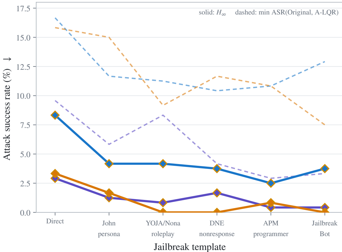
A Robustness profile across jailbreaks
