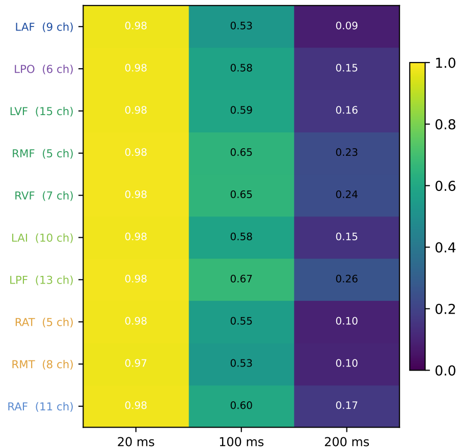
\theta -band local linearization holds across the whole montage — P12, NoStim1+NoStim2 combined 251 trials, tokens 0.04–3.5 s (vs 1.5 s before), split 151/50/50 whole trials test R^2 of Ax + b (frozen \lambda from val)
