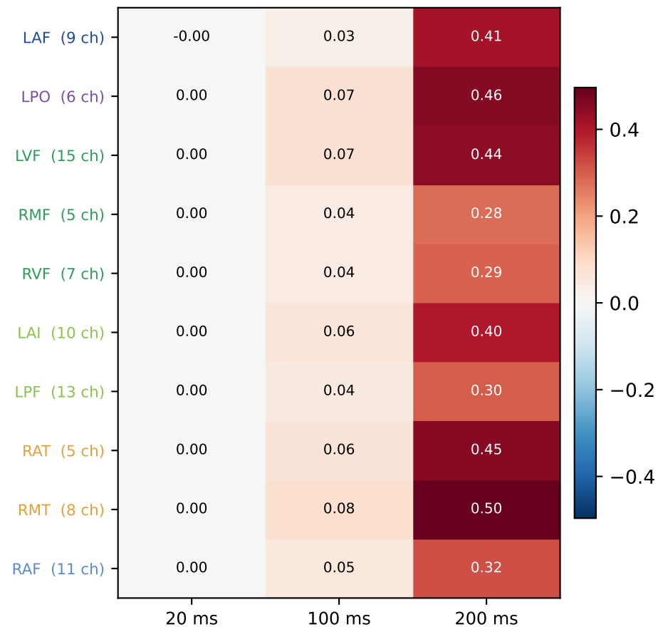
\theta -band local linearization holds across the whole montage — P12, NoStim1+NoStim2 combined 251 trials, tokens 0.04–3.5 s (vs 1.5 s before), split 151/50/50 whole trials test R^2 of Ax + b (frozen \lambda from val)
