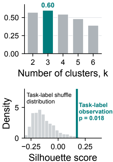
Silhouette score
