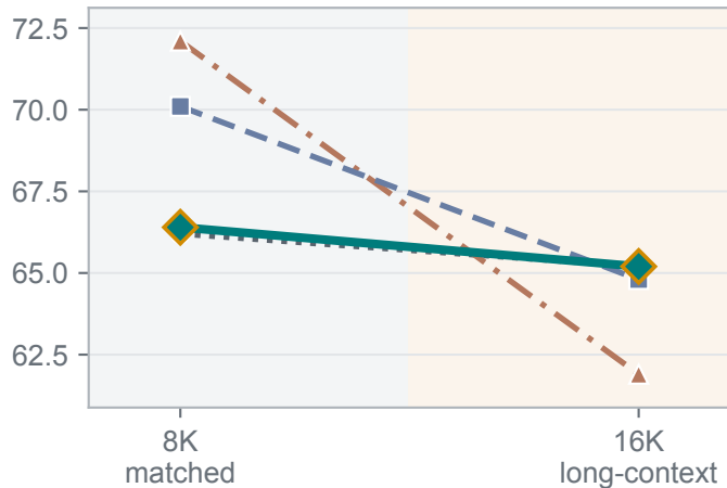
Answer recall (%)
