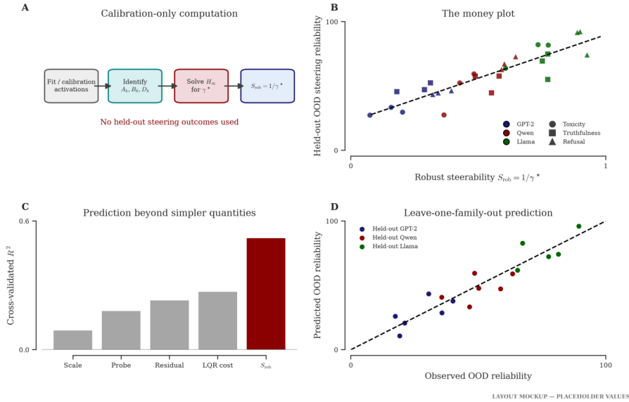
Figure 5 — OOD benchmark
