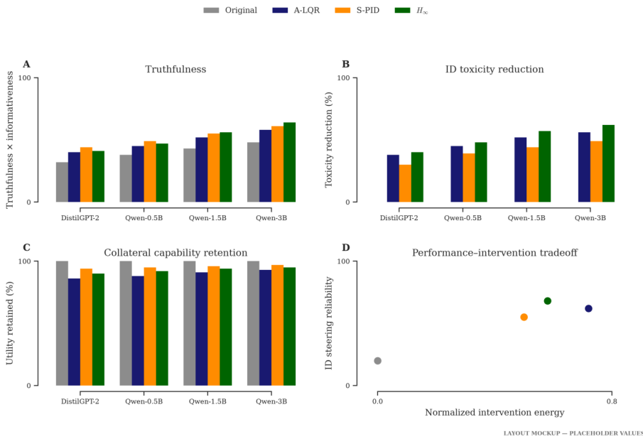
Figure 4 — ID benchmark
