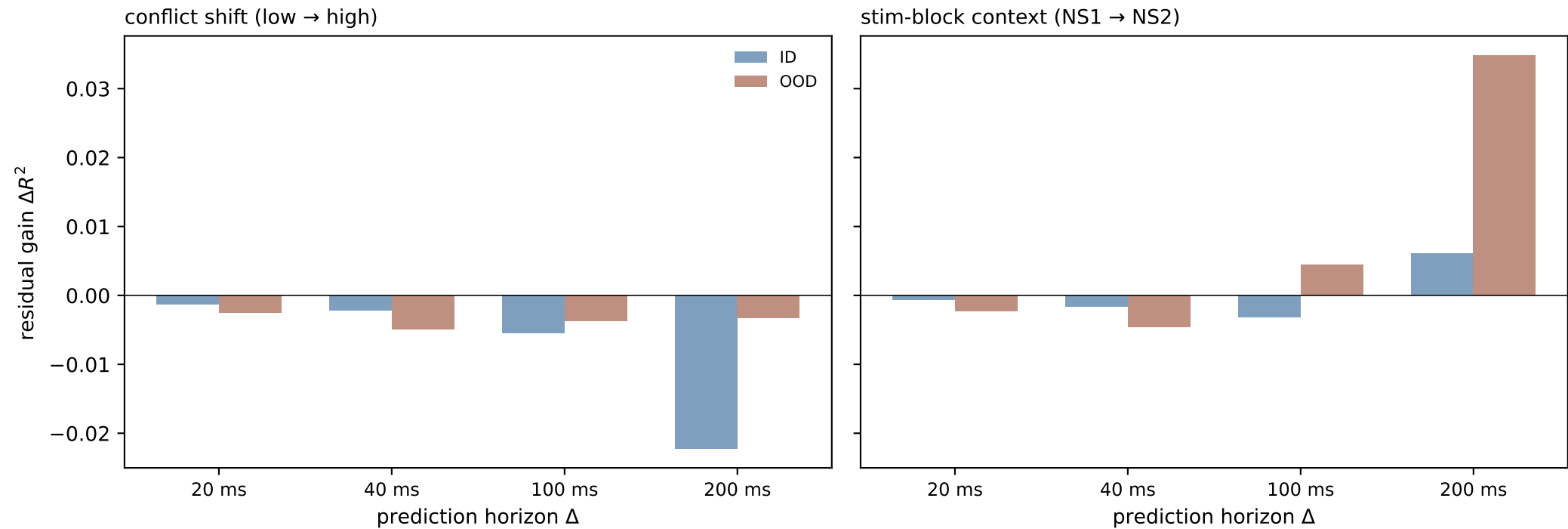
Panel E — does the learned residual g(x) help prediction under OOD? (P12 · LVF · \theta )
