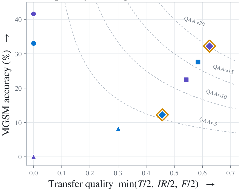
A Capability-steering trade-off
