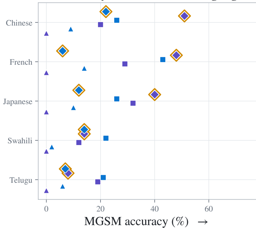
B Accuracy across transfer languages
