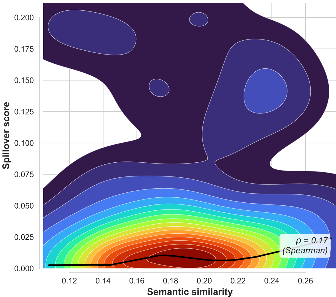
Semantic similarity predicts spillover (llama8b)
