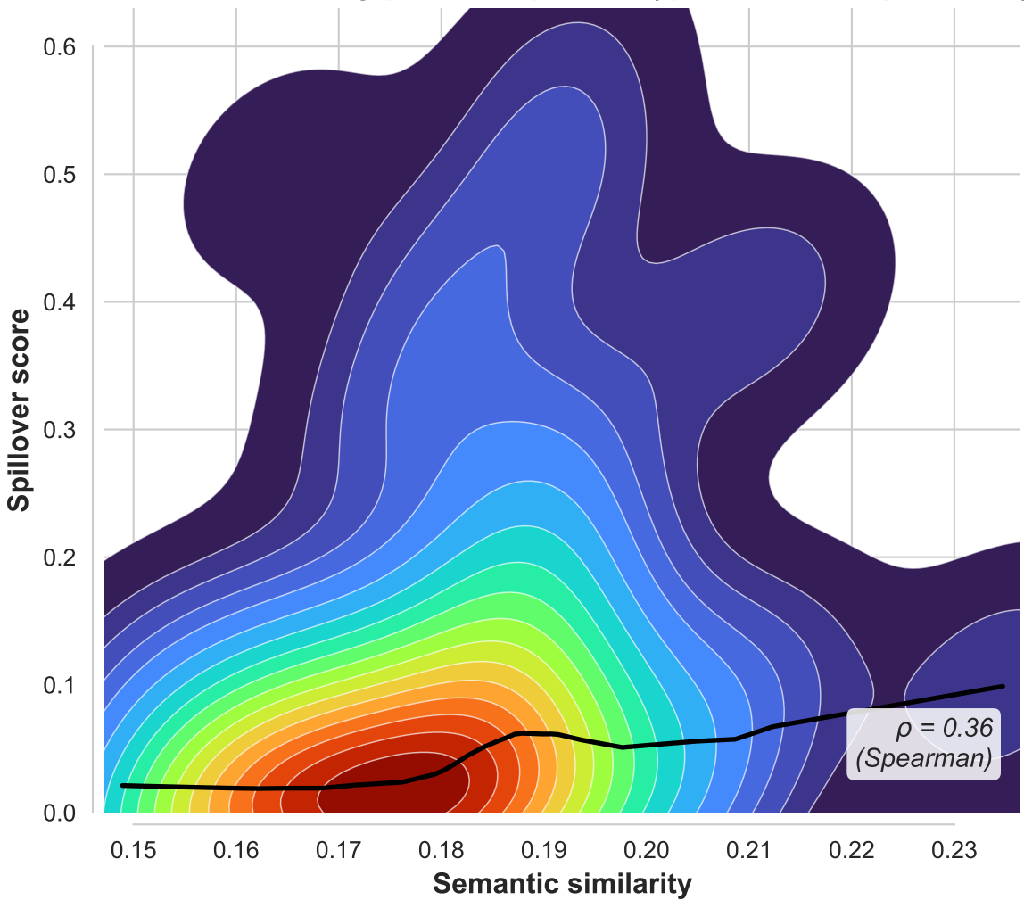
Semantic similarity predicts spillover (qwen7b, conceptvectors)
