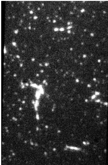
Motor proteins
