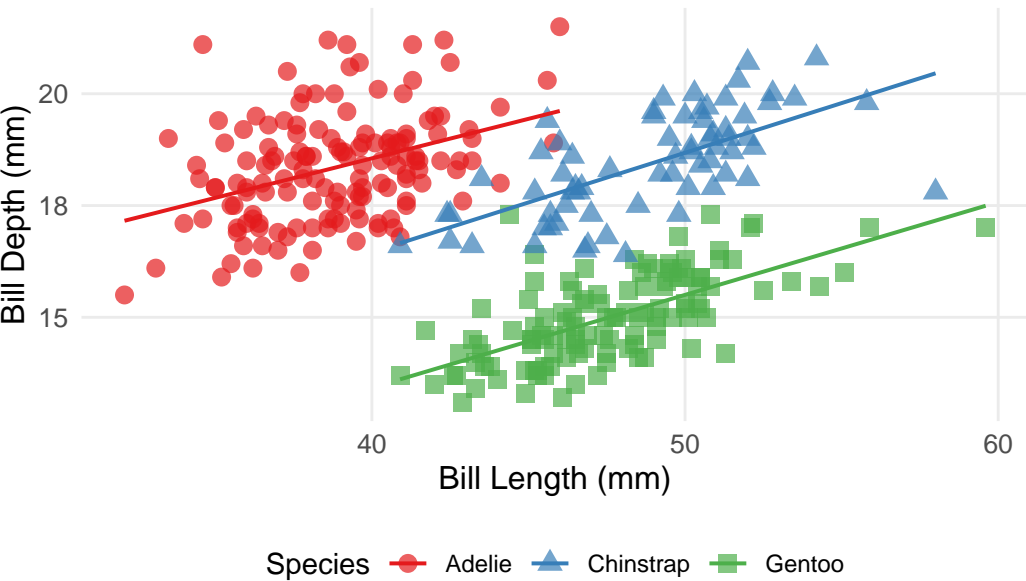
Bill Depth vs Length by Species (R)
