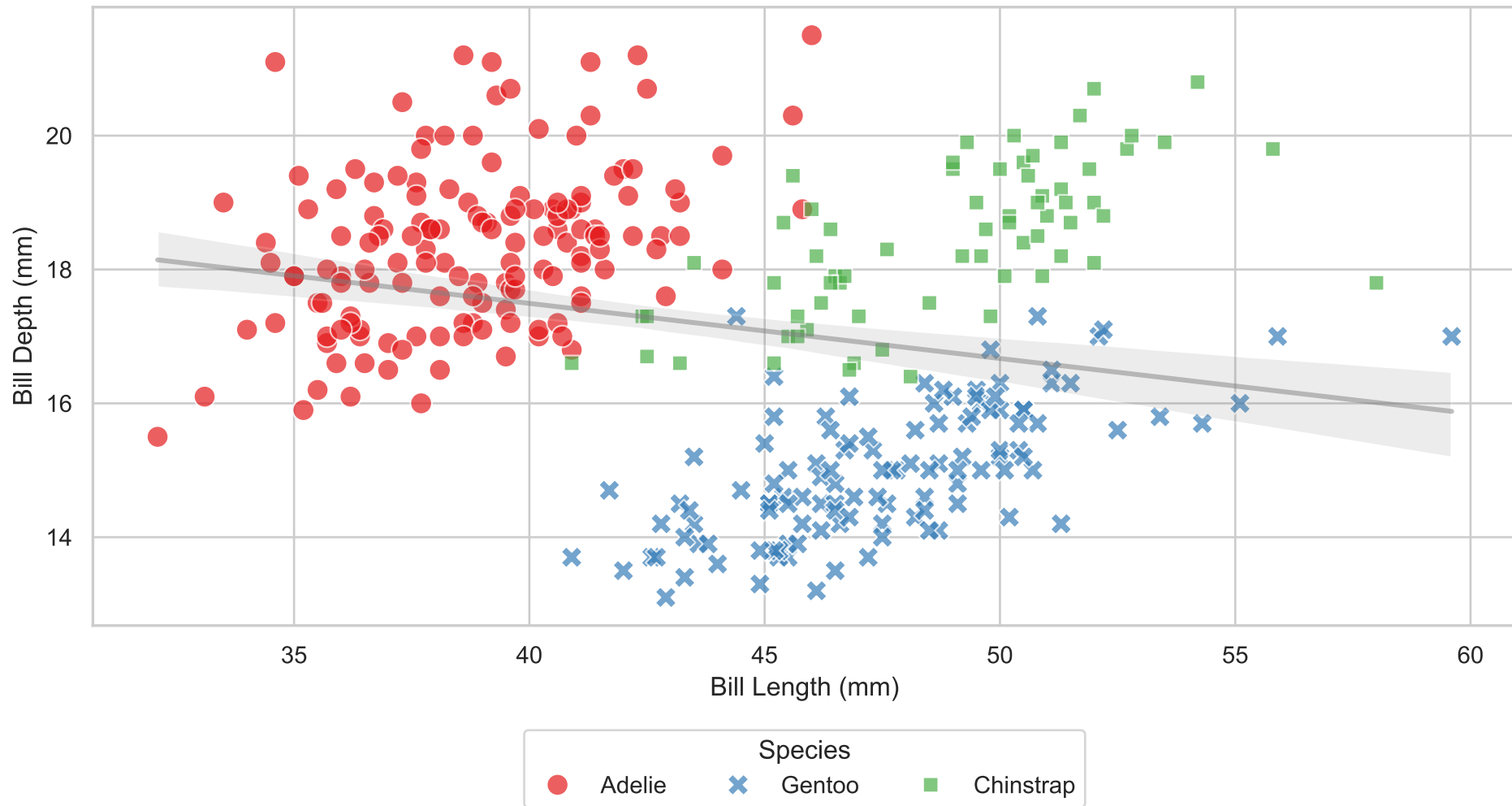
Bill Depth vs Length by Species (Python)
