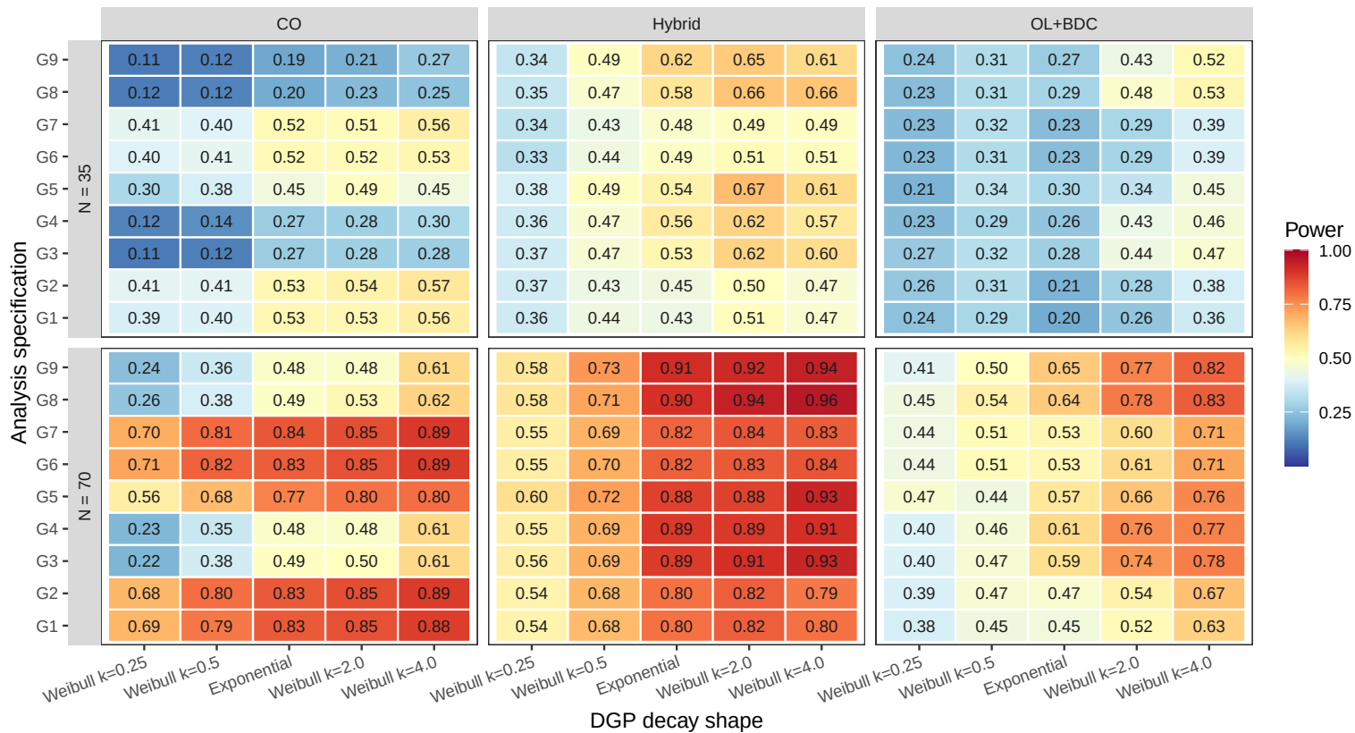
C: Effect of DGP decay shape on power ( c_{bm} = 0.45 , t_{1/2} = 1 )
