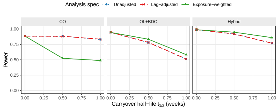
Figure 1: Power versus carryover half-life under the exponential DGP, stratified by analysis specification. Unadjusted and Lag-adjusted are indistinguishable throughout, their curves overlapping in all three panels. Exposure-weighted retains a modest advantage in the Hybrid and OL+BDC designs at t_{1/2} = 1.0 weeks, but is markedly inferior under the crossover (CO) design.
