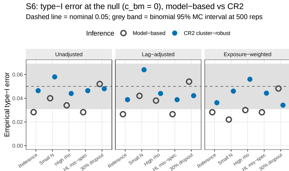
Figure 4: Empirical Type I error at the null ( c_{bm} = 0 ) under model-based and CR2 cluster-robust inference, across the five S6 stress cells and the three specifications. The model-based test (open) is conservative (near 0.03); CR2 (filled) is restored to the nominal 0.05 (dashed), within the binomial Monte Carlo band (gray). 500 null replicates per cell.
