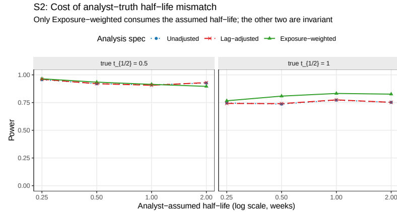
Figure 6: Power as the analyst’s assumed half-life departs from the true DGP half-life. Only Exposure-weighted consumes the assumed half-life; Unadjusted and Lag-adjusted are invariant to it by construction and appear as flat reference lines.
