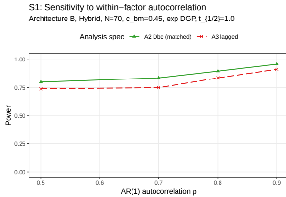
Figure 5: Power by analysis specification across AR(1) autocorrelation \rho \in \{0.5, 0.7, 0.8, 0.9\} , Architecture B.
