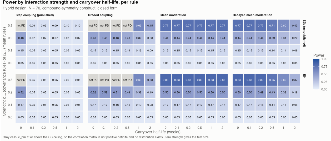
Figure 3: Closed-form power of the paired-difference statistic by interaction strength ( c_{bm} for the covariance rules, \beta_{bm} for the mean rules) and carryover half-life, in the layout of RH's Figure 4B: published step coupling, graded coupling, mean moderation and decayed mean moderation. Upper row: E9b, which counts baseline as an off-drug visit as RH's analysis does; lower row: E9. Gray cells: c_{bm} at or above the compound-symmetry ceiling, where the correlation matrix is not positive definite. Hybrid design, N = 70 , compound symmetry.
