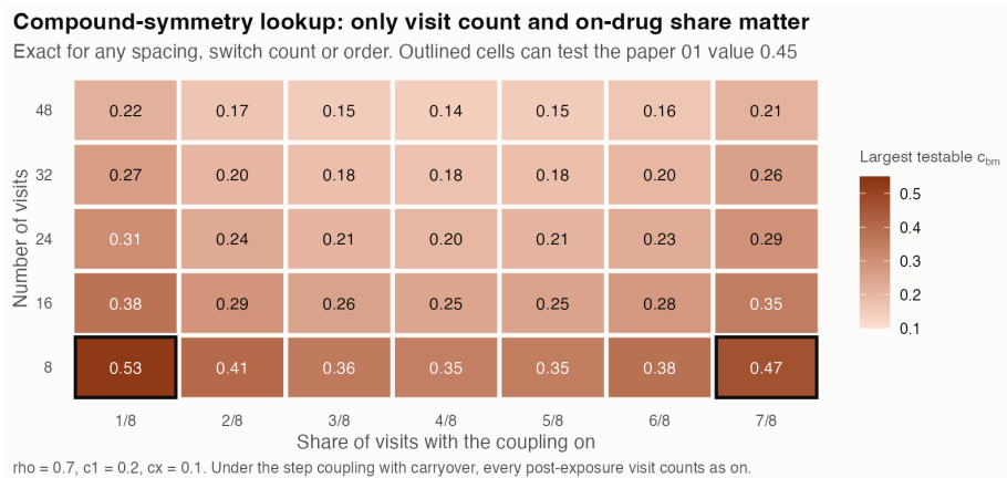
Figure 4: Compound-symmetry lookup by number of visits and on-drug share
