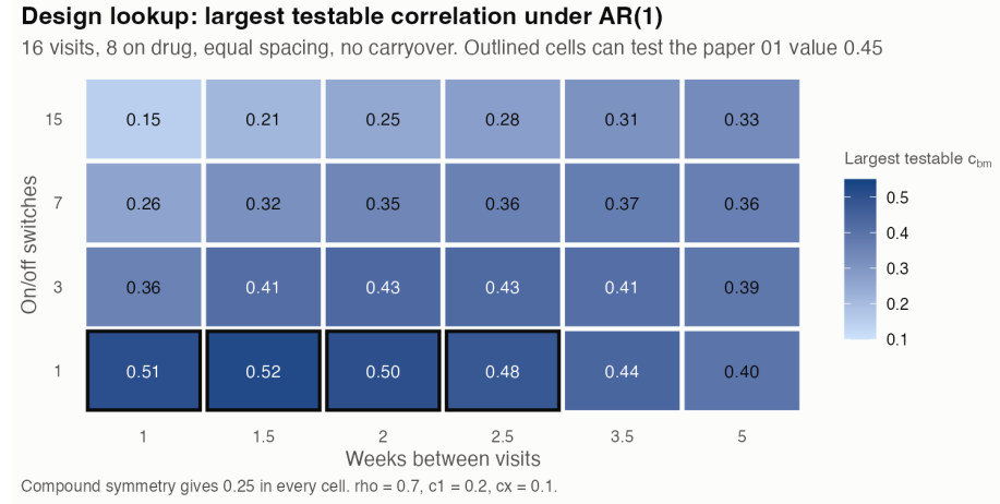
Figure 9: Design lookup for spacing and switches under AR(1)
