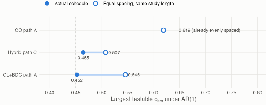
Figure 10: Paper 01 schedules against evenly spaced counterparts
