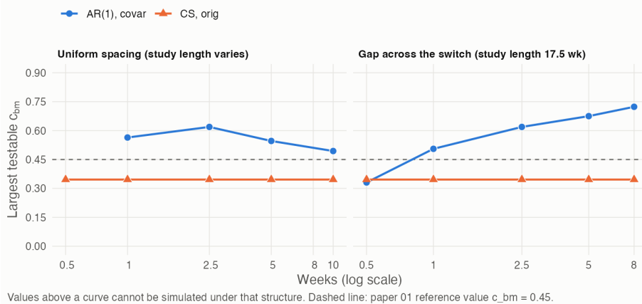
Figure 7: Largest testable c_{bm} by visit spacing
