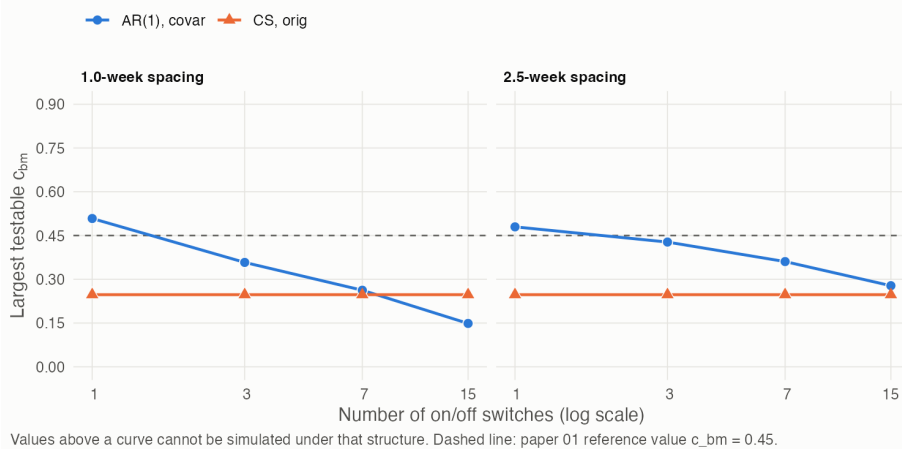
Figure 6: Largest testable c_{bm} by number of switches
