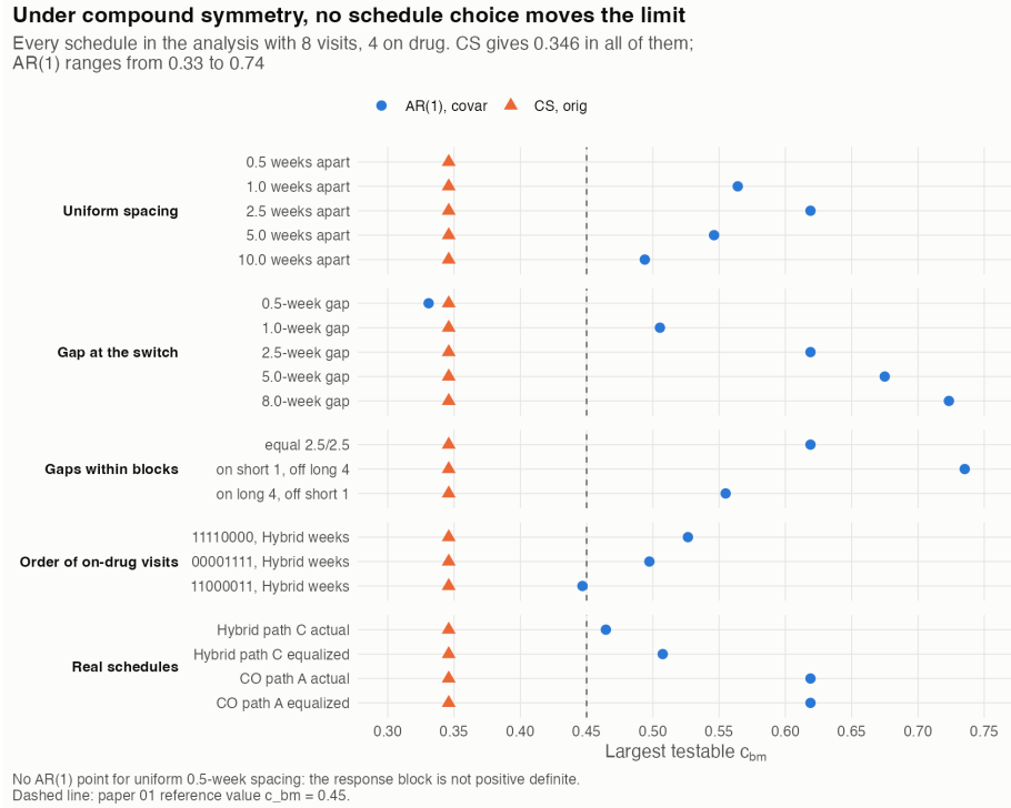
Figure 3: Invariance of the compound-symmetry limit to schedule design
