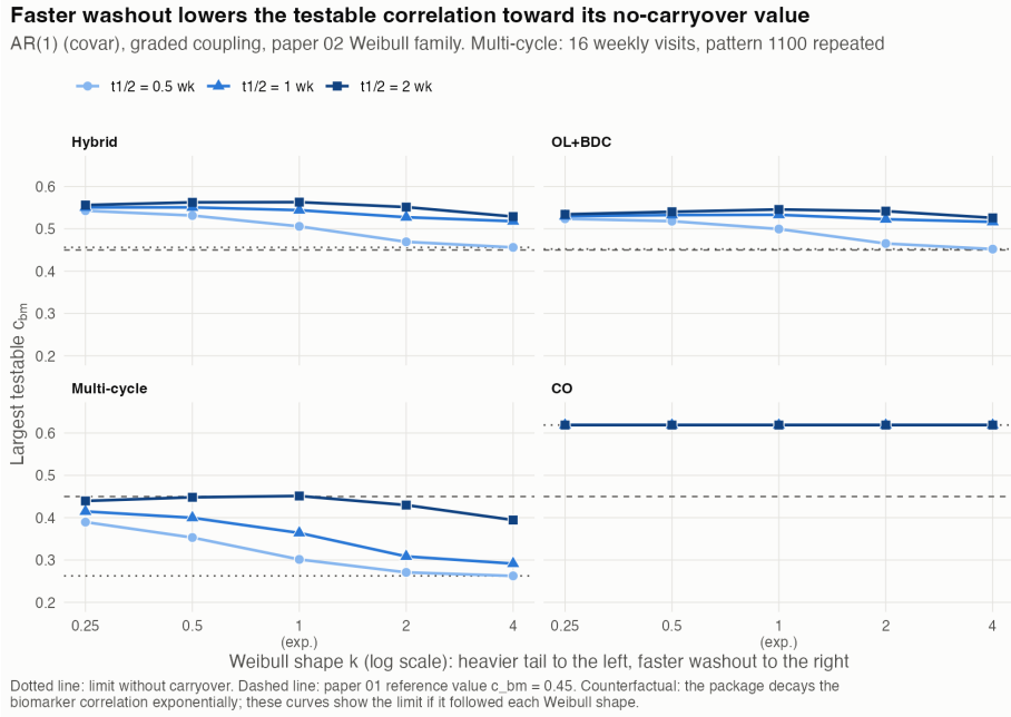
Figure 11: Largest testable c_{bm} by Weibull decay shape
