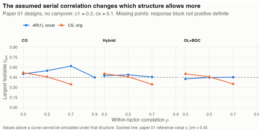
Figure 2: Largest testable c_{bm} by within-factor correlation
