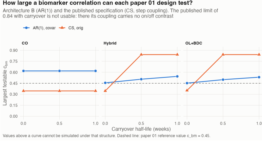
Figure 1: Largest testable c_{bm} for the paper 01 designs
