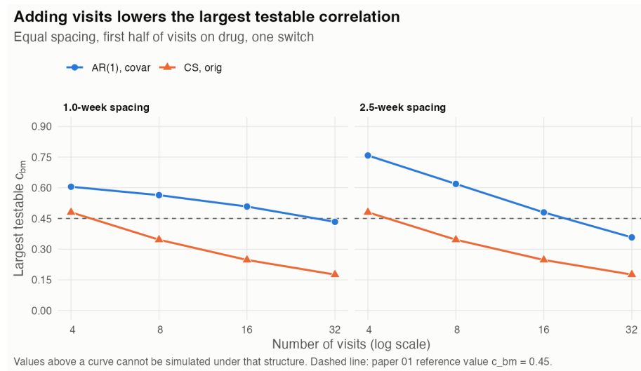
Figure 5: Largest testable c_{bm} by number of visits
