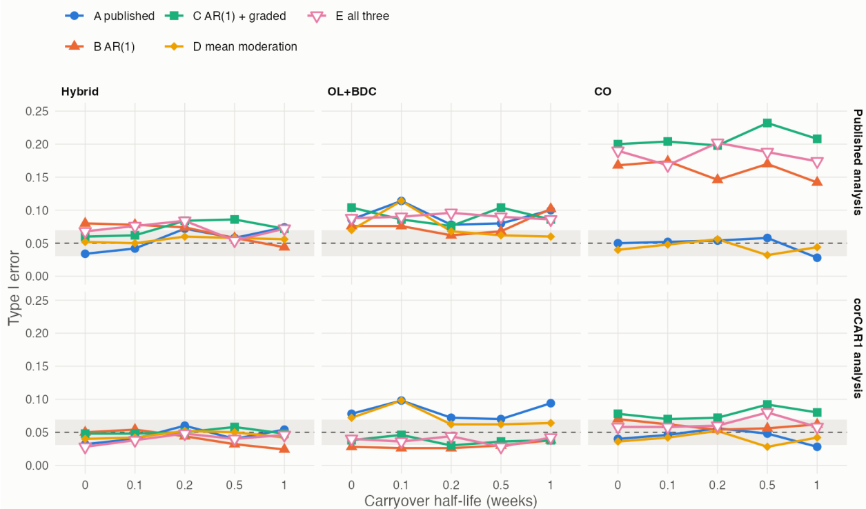
Figure 1: Type I error by configuration and carryover
