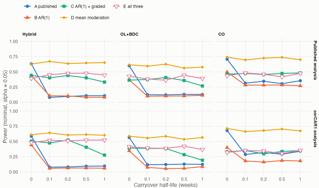
Figure 2: Power by configuration and carryover
