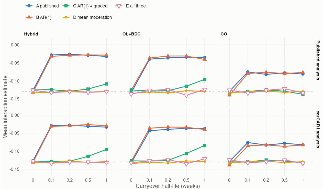
Figure 3: Mean interaction estimate by configuration and carryover
