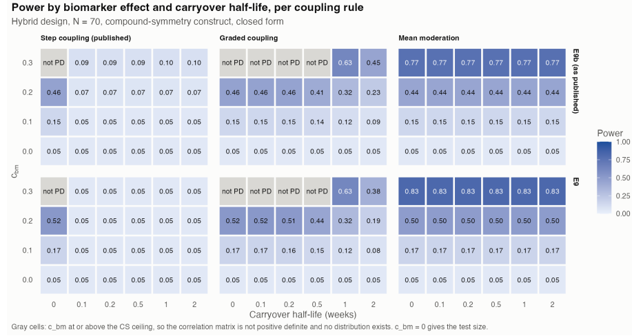
Figure 3: Power by biomarker effect and carryover half-life
