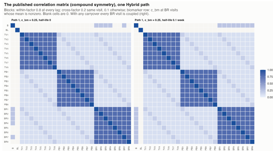
Figure 6: The published correlation matrix for path 1 at c_{\text{bm}} = 0.25 , without carryover (left) and with a 0.1-week half-life (right).
