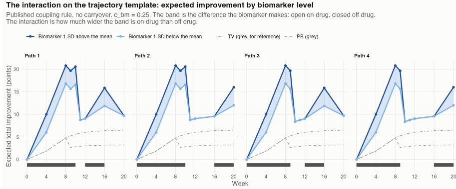
Figure 4: The template conditioned on the biomarker: expected total improvement at one SD above and one SD below the biomarker mean, published coupling, no carryover.
