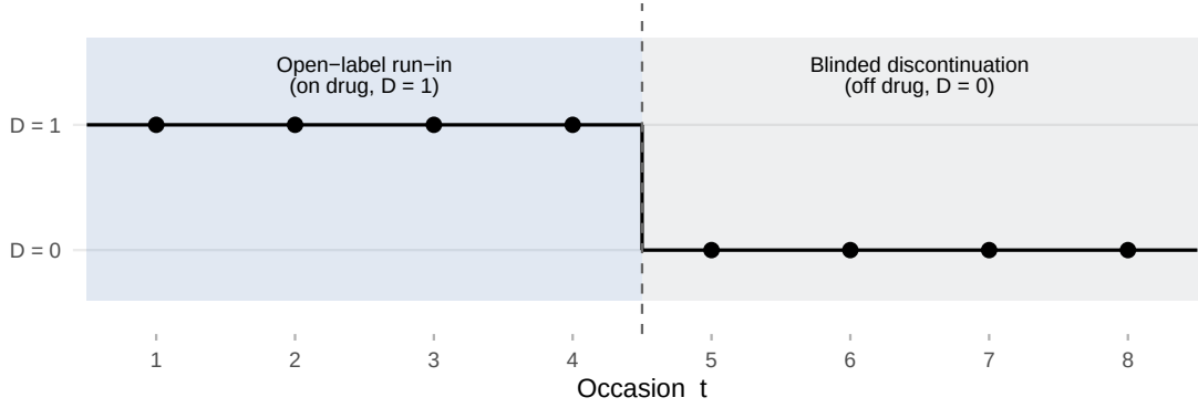
Figure 1: The simplest hybrid design with p = 4 on-drug and q = 4 off-drug occasions. Every participant begins on active drug (open-label run-in, drug indicator D_t = 1 ) and is then taken off drug under blinding (discontinuation, D_t = 0 ) at the dashed transition. Filled points mark the measurement occasions; the within-participant on/off contrast of these occasions, regressed on the biomarker across participants, identifies the interaction \theta .
