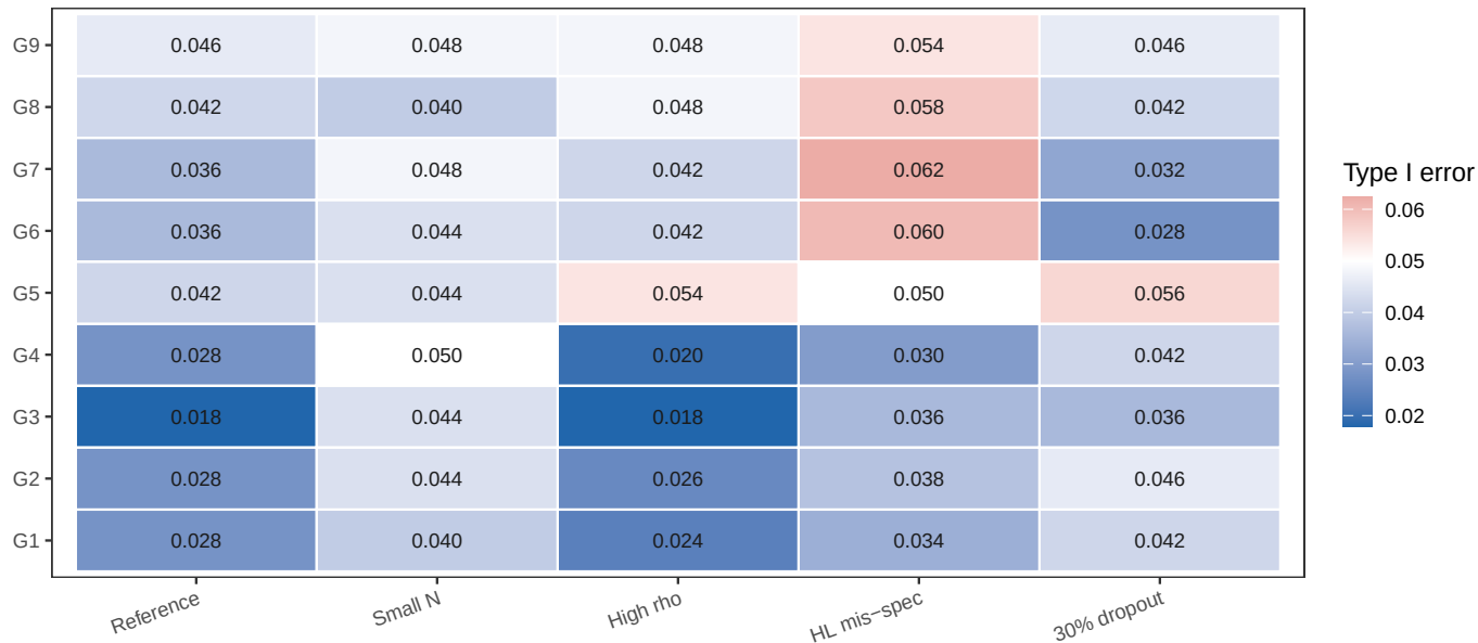
S6 (G1–G9): Type I error across five stress cells
