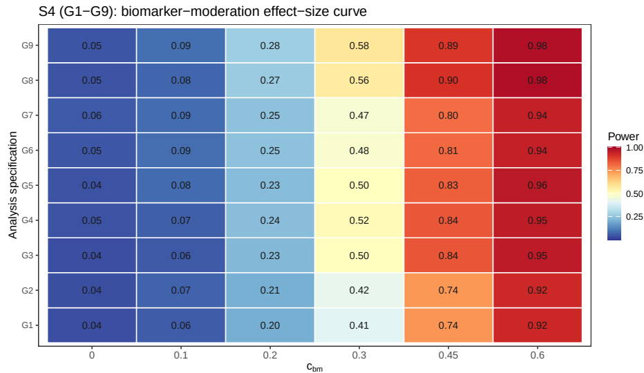
Figure 9: Block S4 extended to all nine G1-G9 specifications ( n_{sim} = 500 ).
