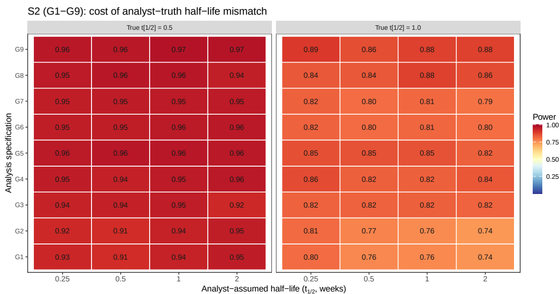
Figure 6: Block S2 extended to all nine G1-G9 specifications ( n_{sim} = 500 ).
