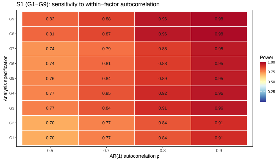
Figure 3: Block S1 extended to all nine G1-G9 specifications ( n_{sim} = 500 ).
