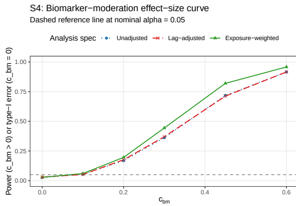
Figure 8: Power across the biomarker-moderation effect-size range c_{bm} \in \{0, 0.10, 0.20, 0.30, 0.45, 0.60\} under the covariance-moderation architecture. The c_{bm} = 0 point is the null for Type I verification.
