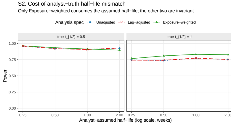
Figure 6: Power as the analyst's assumed half-life departs from the true DGP half-life. Only Exposure-weighted consumes the assumed half-life; Unadjusted and Lag-adjusted are invariant to it by construction and appear as flat reference lines.
