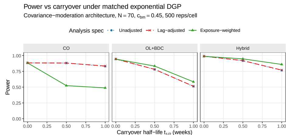
Figure 1: Power versus carryover half-life under the exponential DGP, the covariance-moderation architecture, stratified by analysis specification. Unadjusted and Lag-adjusted are indistinguishable throughout, their curves overlapping in all three panels. Exposure-weighted retains a modest advantage in the Hybrid and OL+BDC designs at t_{1/2} = 1.0 weeks, but is markedly inferior under the crossover (CO) design.
