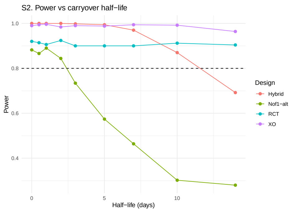
Figure 2: Sensitivity S2: power versus carryover half-life across four designs.
