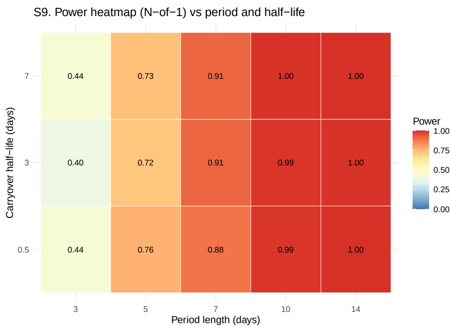
Figure 9: Sensitivity S9: heatmap of N-of-1 power over period length and carryover half-life.
