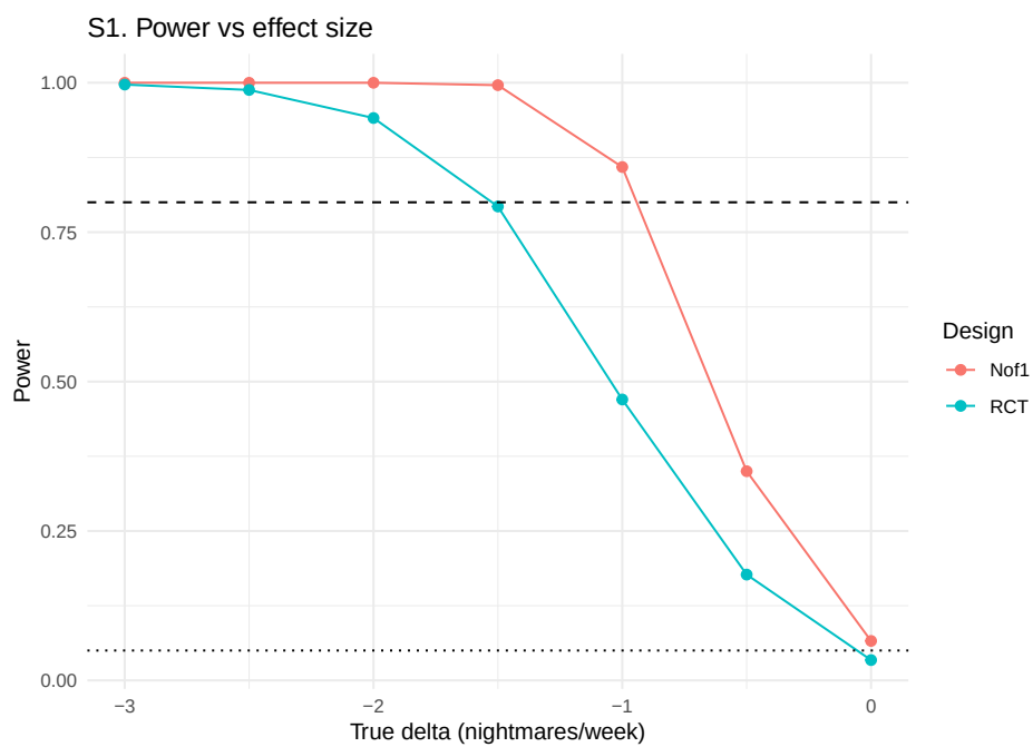
Figure 1: Sensitivity S1: power versus effect-size axis for N-of-1 and parallel RCT.
