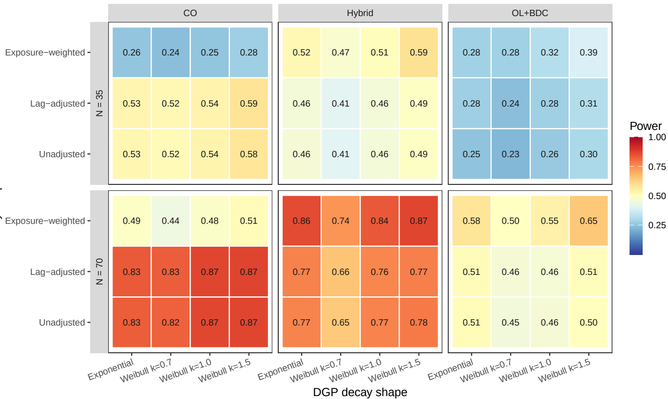
C: Effect of DGP decay shape on power ( c_{bm} = 0.45 , t_{1/2} = 1 )
