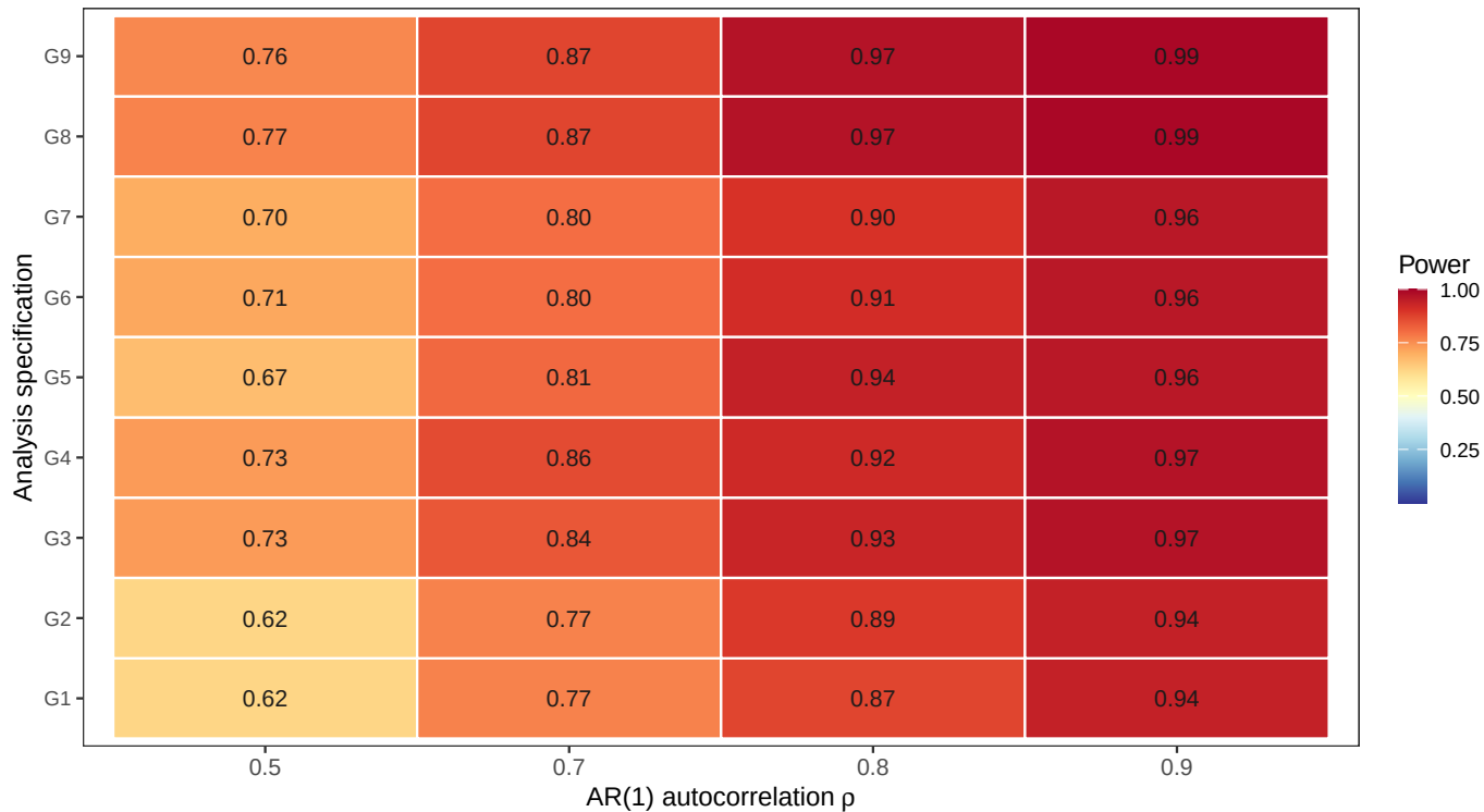
S1 (G1–G9): sensitivity to within-factor autocorrelation
