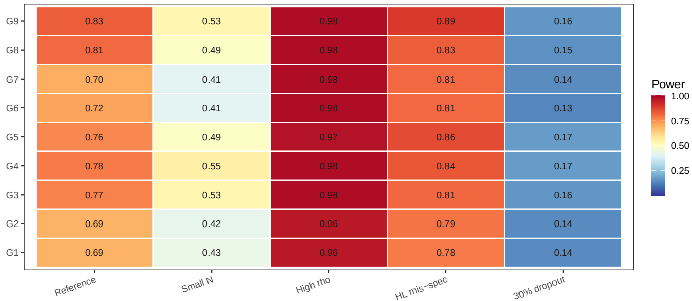
S6 (G1–G9): power across five stress cells
