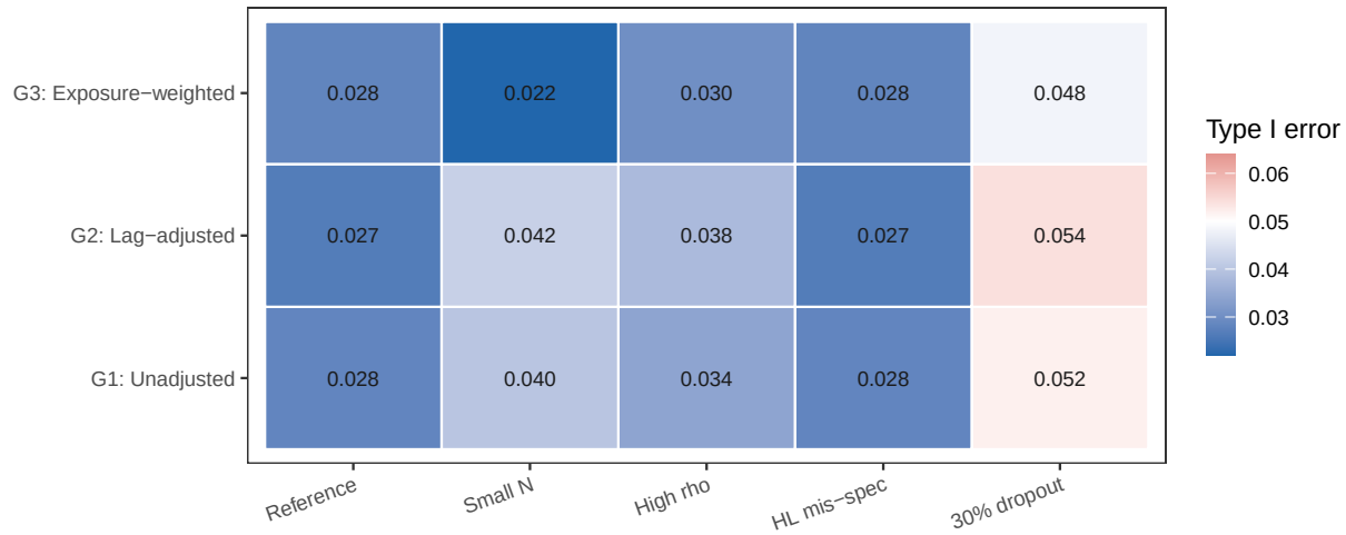
S6 Panel A: model-based Type I error
