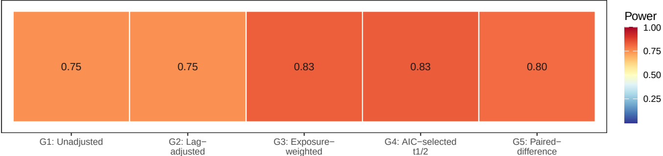
S7: G1–G5 at the Hybrid reference cell
