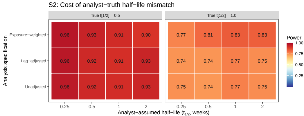
Figure 13: Block S2: power by analyst-assumed half-life and analysis specification, faceted by true half-life, same data as the line plot above.
