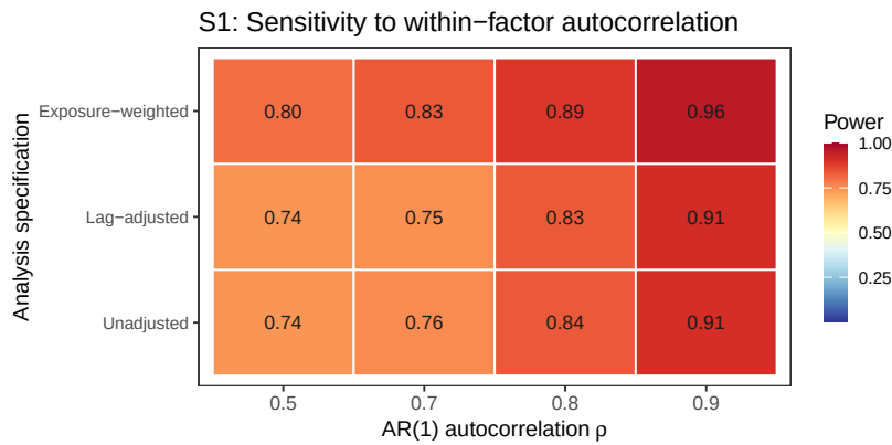
Figure 11: Block S1: power by AR(1) autocorrelation and analysis specification, same data as the line plot above.
