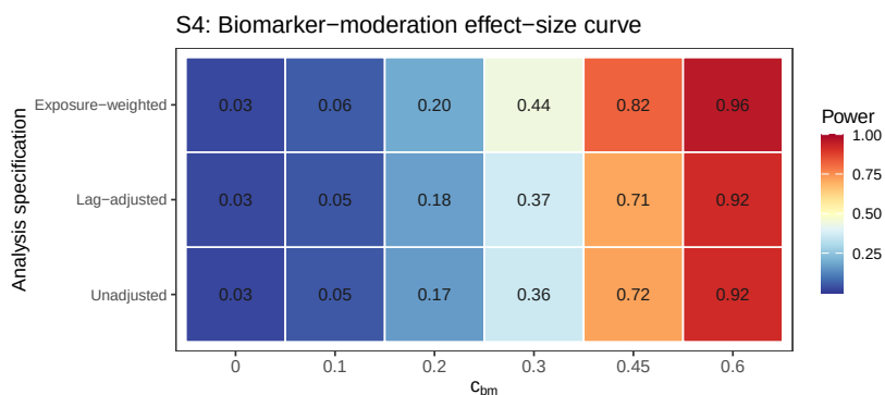
Figure 17: Block S4: power by biomarker-moderation effect size and analysis specification, same data as the line plot above.
