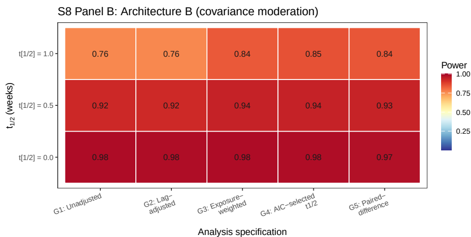
Figure 20: Block S8, Panel B (Architecture B, covariance moderation): power by carryover half-life (rows) and analysis specification (columns). Same data as the Architecture B rows of the table above. Not directly comparable to Panel A in absolute terms (Section 3.6).
