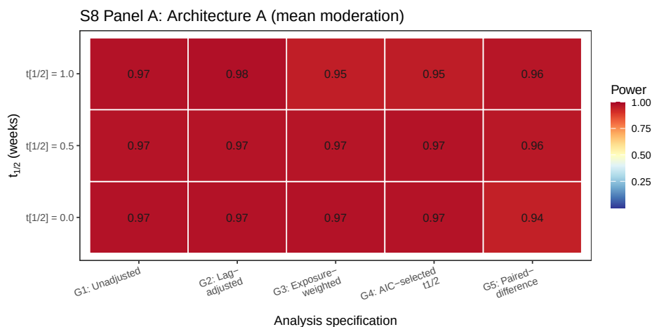
Figure 19: Block S8, Panel A (Architecture A, mean moderation): power by carryover half-life (rows) and analysis specification (columns). Same data as the Architecture A rows of the table above.
