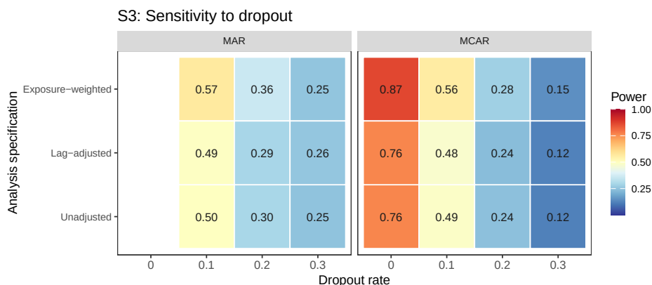
Figure 15: Block S3: power by dropout rate and analysis specification, faceted by dropout mechanism, same data as the line plot above. The MAR arm has no 0% cell (Section 3.6); it shares the MCAR reference cell.
