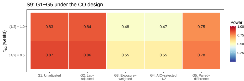
Figure 21: Block S9: power under the CO design at two true half-lives, all five G1-G5 specifications.
