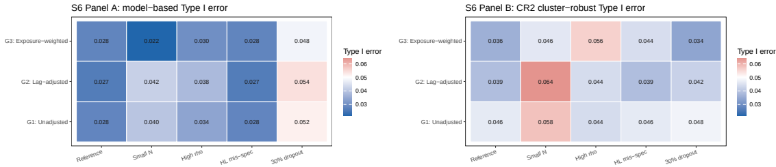
Figure 9: Same data as the dot plot above, as two annotated heatmaps (model-based, CR2) sharing one diverging scale centered at nominal 0.05.
