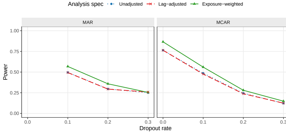
Figure 14: Power at dropout rates \in \{0, 0.1, 0.2, 0.3\} under MCAR and MAR mechanisms.
