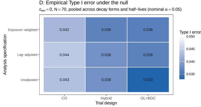
Figure 7: Same data as the boxplot above, as an annotated heatmap of the mean Type I error per design x specification cell (diverging scale centered at nominal 0.05: blue = conservative, red = anti-conservative).
