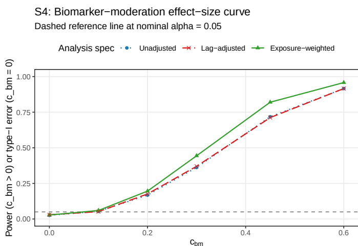
Figure 16: Power across the biomarker-moderation effect-size range c_{bm} \in \{0, 0.10, 0.20, 0.30, 0.45, 0.60\} . The c_{bm} = 0 point is the null for Type I verification.
