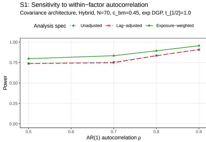
Figure 10: Power by analysis specification across AR(1) autocorrelation \rho \in \{0.5, 0.7, 0.8, 0.9\} .
