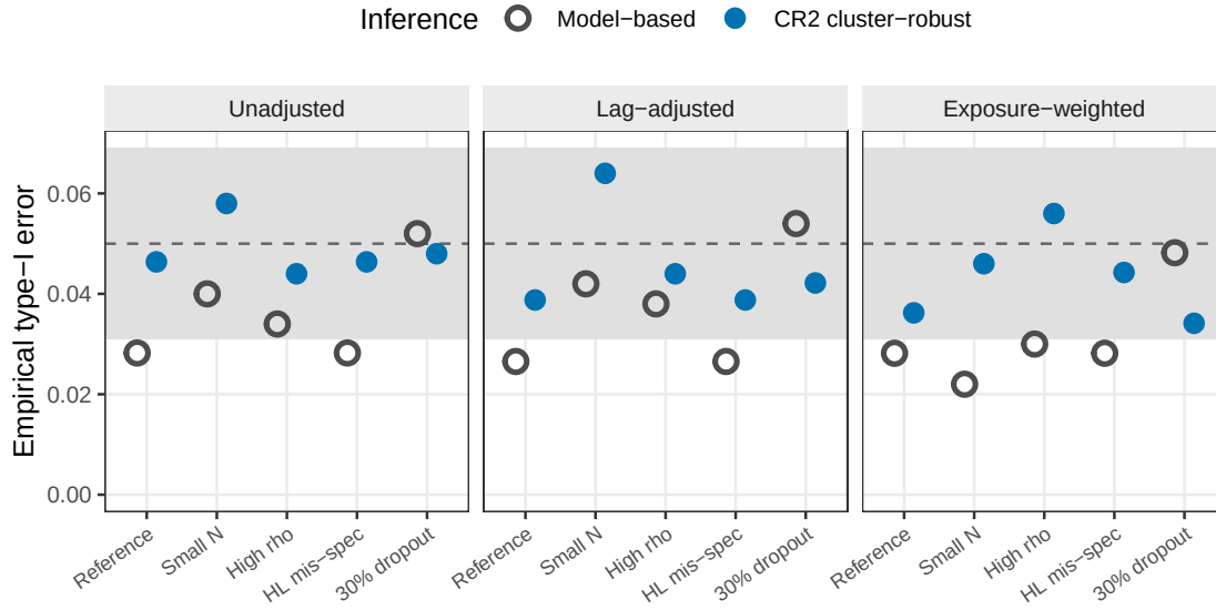
Figure 8: Empirical Type I error at the null ( c_{bm} = 0 ) under model-based and CR2 cluster-robust inference, across the five S6 stress cells and the three specifications. The model-based test (open) is conservative (near 0.03), and CR2 (filled) is restored to the nominal 0.05 (dashed), within the binomial Monte Carlo band (grey). 500 null replicates per cell.
