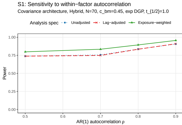
Figure 10: Power by analysis specification across AR(1) autocorrelation \rho \in \{0.5, 0.7, 0.8, 0.9\} .
