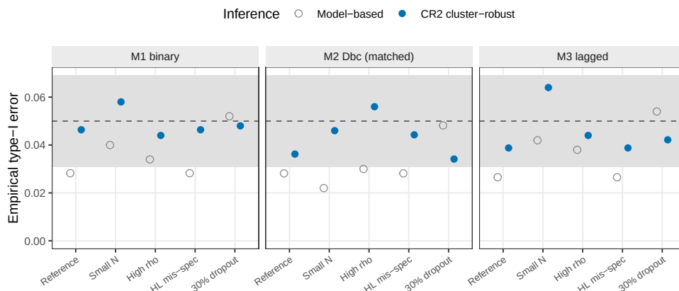
Figure 4: Empirical Type I error at the null ( c_{bm} = 0 ) under the model-based and CR2 cluster-robust inference, across the five S6 cells and the three specifications. The model-based test (open circles) is conservative, sitting near 0.03; the CR2 test (filled) is restored to the nominal 0.05 (dashed line), within the binomial Monte Carlo band (gray). 500 null replicates per cell.
