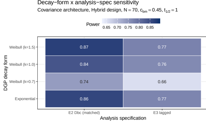
Figure 2: Power at the critical cell ( t_{1/2} = 1.0 weeks, the covariance-moderation architecture, Hybrid design, N = 70 , c_{bm} = 0.45 ) across DGP decay forms (rows) and analysis specifications (columns). Under the heavy-tailed Weibull DGP ( k = 0.7 ), E2’s advantage over E3 narrows because its assumed exponential decay no longer matches truth. The fill scale is stretched to the observed power range (0.66-0.87), not the full [0,1] range, so that these cell-to-cell differences are visible; the absolute shading should not be compared to other figures in this manuscript.
