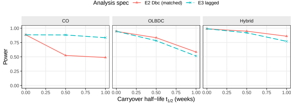
Figure 1: Power versus carryover half-life under the exponential DGP, the covariance-moderation architecture, stratified by analysis specification. E2 retains a modest advantage over E3 in the Hybrid and OL+BDC designs at t_{1/2} = 1.0 weeks, but is dominated by E3 under the crossover (CO) design.
