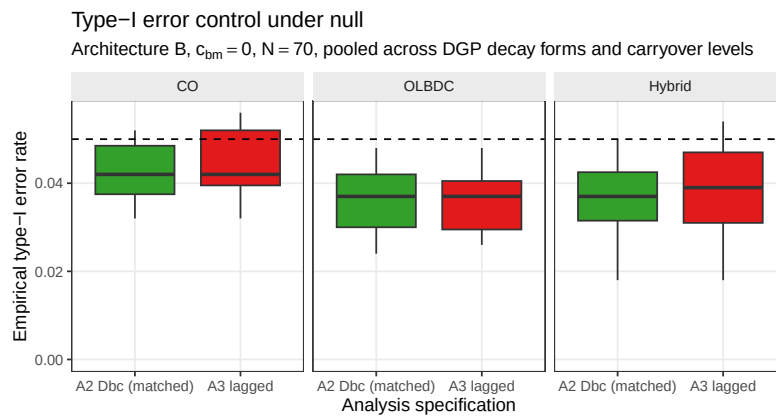
Figure 3: Empirical Type I error rates under the null ( c_{bm} = 0 ), Architecture B, pooled across DGP decay forms and carryover half-lives, stratified by design and analysis specification. Boxplots cover the distribution across cells at N = 70 ; the dashed reference line marks the nominal 0.05 level.
