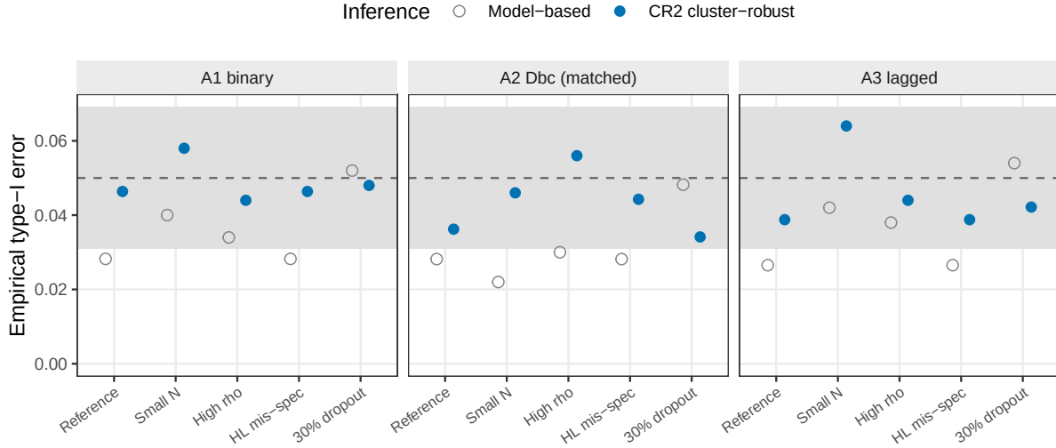
Figure 10: Empirical type-I error at the null ( c_{bm} = 0 ) under the model-based and CR2 cluster-robust inference, across the five S6 cells and the three specifications. The model-based test (open) is conservative (near 0.03); CR2 (filled) is restored to the nominal 0.05 (dashed), within the binomial Monte Carlo band (grey). 500 null replicates per cell.
