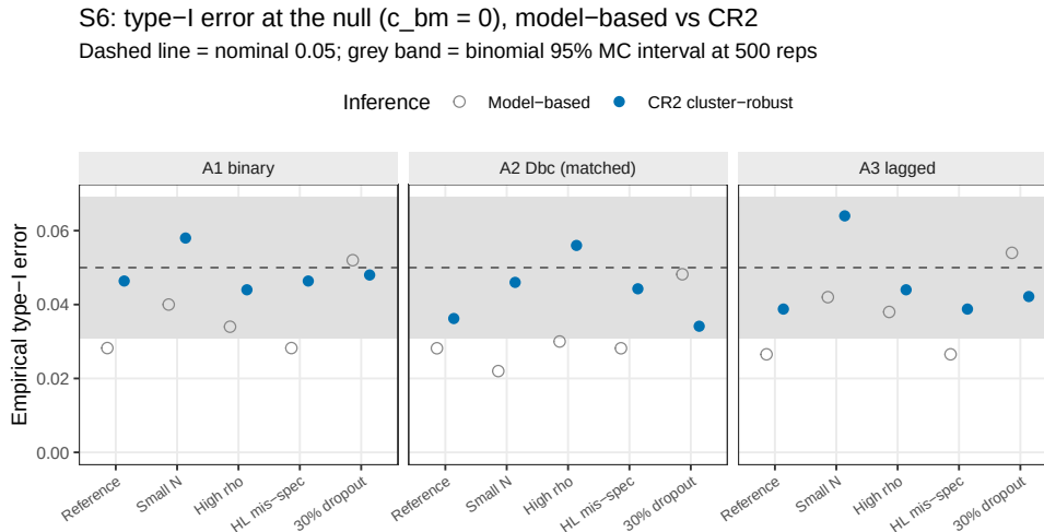
Figure 10: Empirical type-I error at the null ( c_{bm} = 0 ) under the model-based and CR2 cluster-robust inference, across the five S6 cells and the three specifications. The model-based test (open circles) is conservative, sitting near 0.03; the CR2 test (filled) is restored to the nominal 0.05 (dashed line), within the binomial Monte Carlo band (grey). 500 null replicates per cell.
