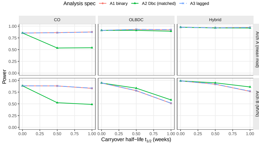
Power vs carryover under matched exponential DGP N = 70, c_{bm} = 0.45 , 500 reps/cell
