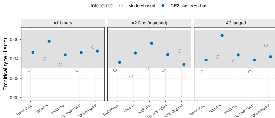
S6: type-I error at the null ( c_{bm} = 0 ), model-based vs CR2 Dashed line = nominal 0.05; grey band = binomial 95% MC interval at 500 reps
