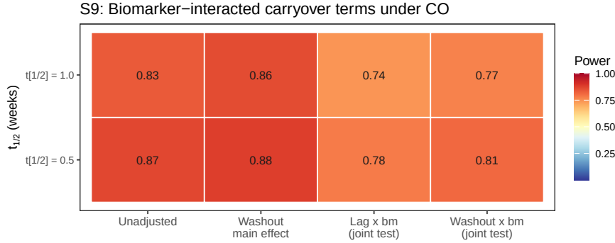
Figure 19: Block S9: power under the CO design at two true half-lives, same four specifications as block S7.
