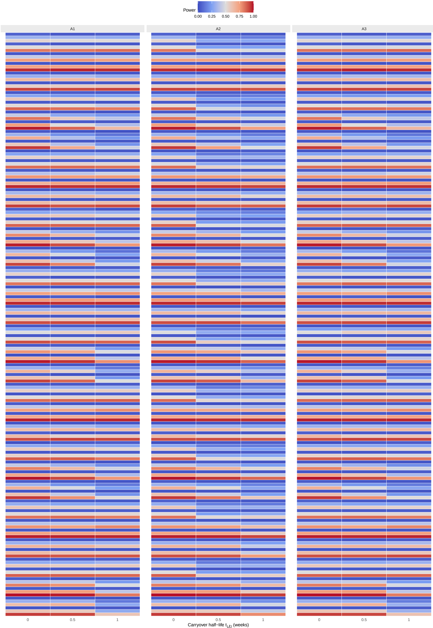
Lasagna plot: power across the 540-cell factorial Each row is a unique cell (decay form, architecture, design, N, c_bm); columns within a panel are carryover half-lives; panels are analysis specifications.
