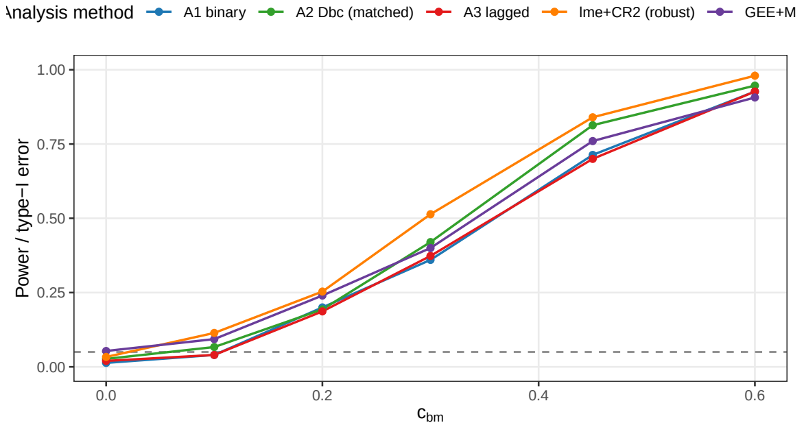
Figure 7: Power across c_{bm} \in \{0, 0.10, 0.20, 0.30, 0.45, 0.60\} , for all five analysis methods. The c_{bm} = 0 point is the null; dashed line at nominal \alpha = 0.05 .
