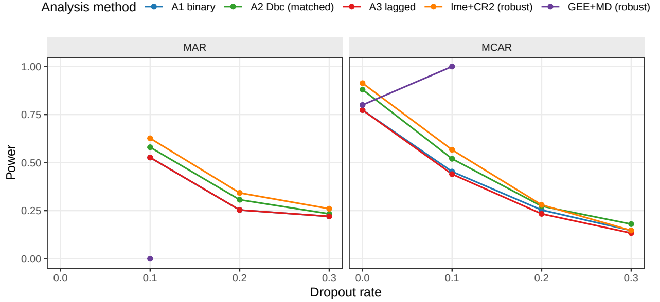
Figure 6: Power at dropout rates \in \{0, 0.1, 0.2, 0.3\} under MCAR and MAR mechanisms. GEE+MD is unreliable here: the Mancl-DeRouen variance (geesmv) fails on the unbalanced clusters that monotone dropout produces, so its dropout points are degenerate or absent. The model-based specifications and lme+CR2 are unaffected.
