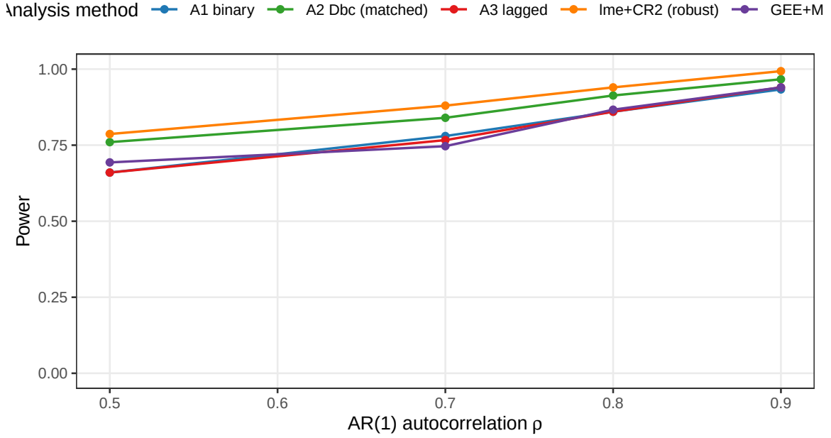
Figure 4: Power by analysis method across AR(1) autocorrelation \rho \in \{0.5, 0.7, 0.8, 0.9\} . Reference: Arch B, Hybrid, N = 70 , c_{bm} = 0.45 , exponential DGP, t_{1/2} = 1.0 weeks.
