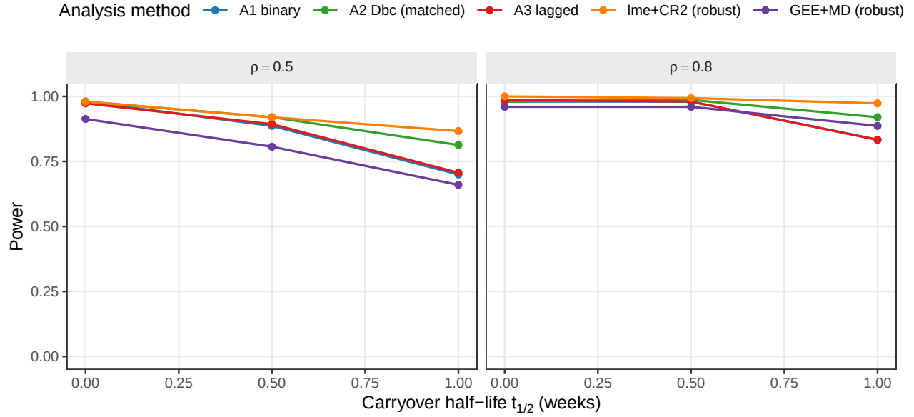
Figure 8: Power across carryover half-lives \{0, 0.5, 1.0\} weeks at \rho \in \{0.5, 0.8\} , for all five analysis methods. Facets by \rho .
