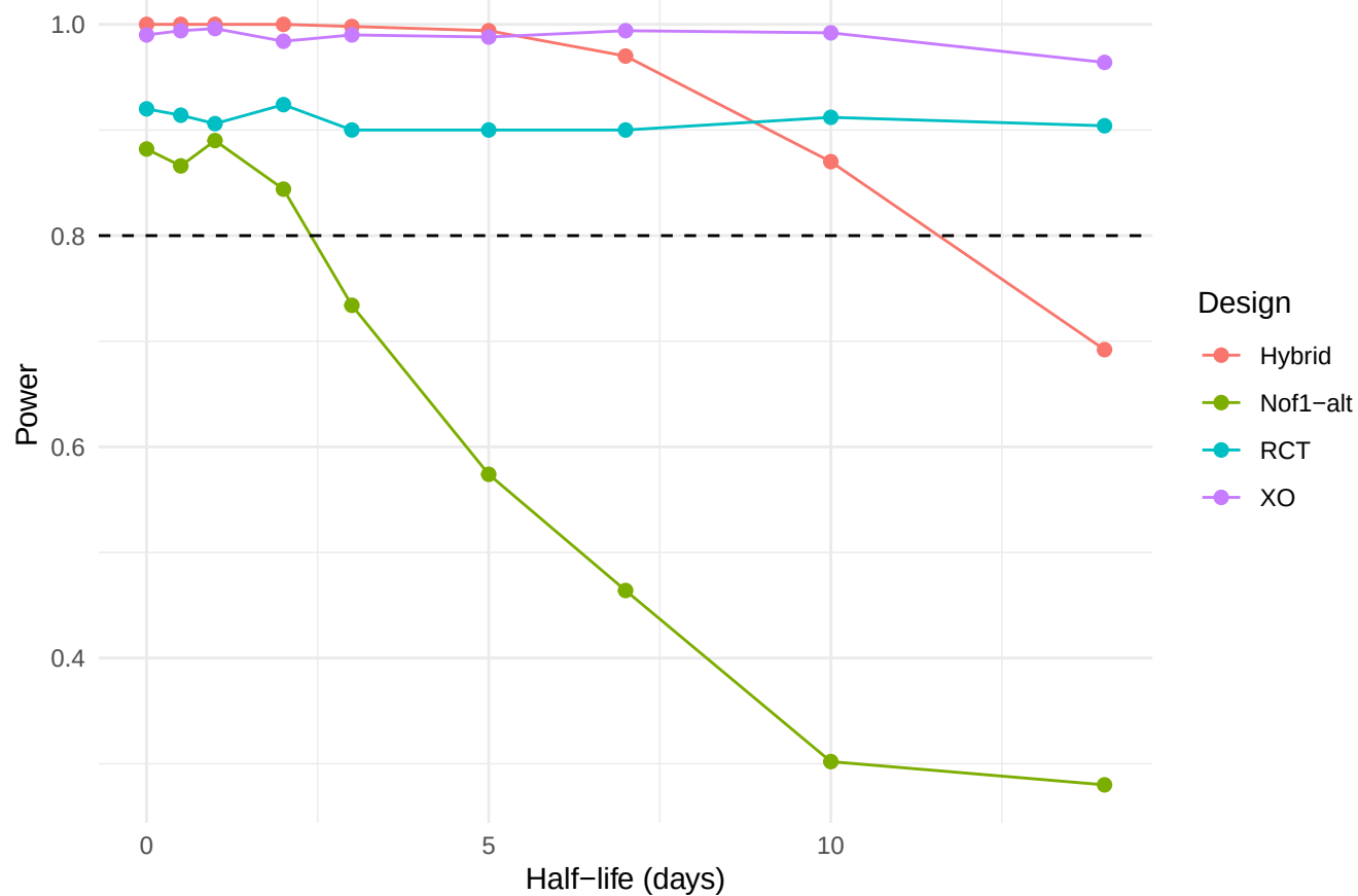
S2. Power vs carryover half-life
