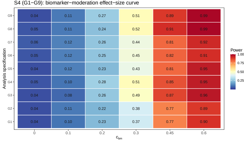
Figure 17: Block S4 extended to all nine G1-G9 specifications (preliminary n_{sim} = 100 ).
