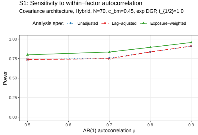
Figure 6: Power by analysis specification across AR(1) autocorrelation \rho \in \{0.5, 0.7, 0.8, 0.9\} .
