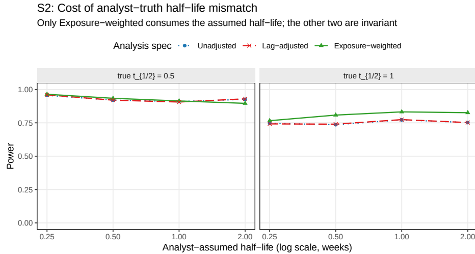
Figure 9: Power as the analyst's assumed half-life departs from the true DGP half-life. Only Exposure-weighted consumes the assumed half-life. Unadjusted and Lag-adjusted are invariant to it by construction and appear as flat reference lines.
