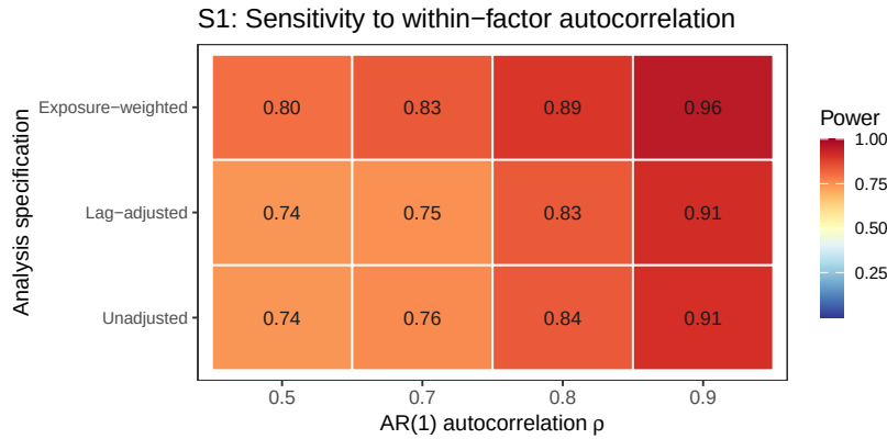
Figure 7: Block S1: power by AR(1) autocorrelation and analysis specification, same data as the line plot above.
