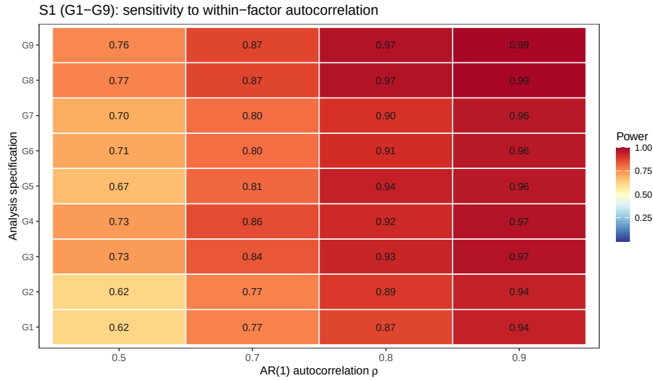
Figure 8: Block S1 extended to all nine G1-G9 specifications (preliminary n_{sim} = 100 ).
