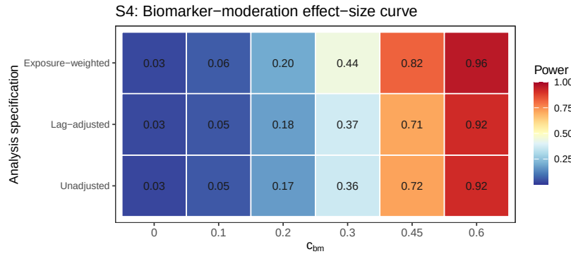
Figure 16: Block S4: power by biomarker-moderation effect size and analysis specification, same data as the line plot above.
