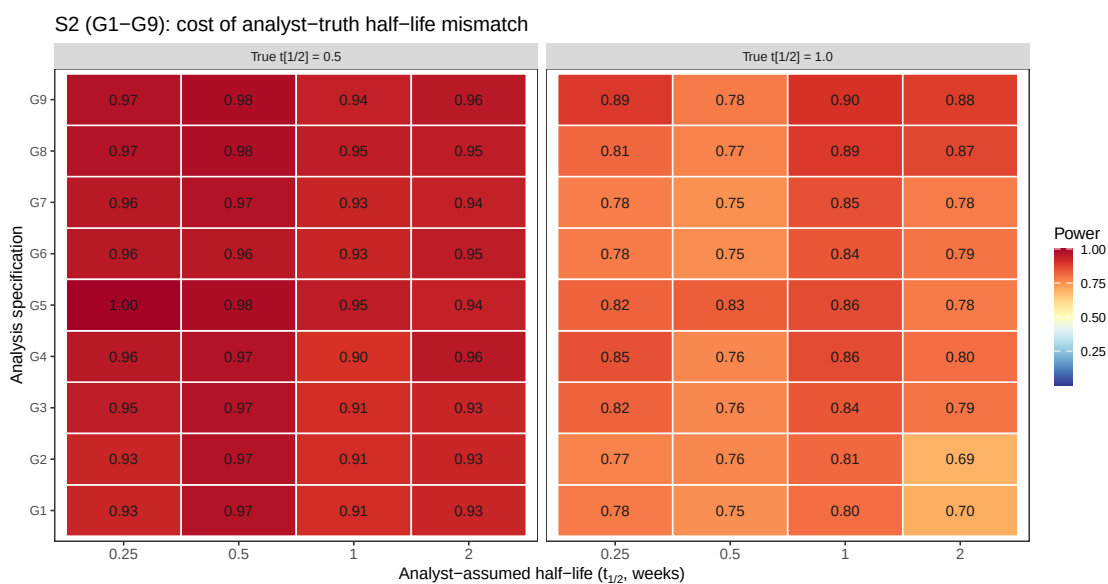
Figure 11: Block S2 extended to all nine G1-G9 specifications (preliminary n_{sim} = 100 ).
