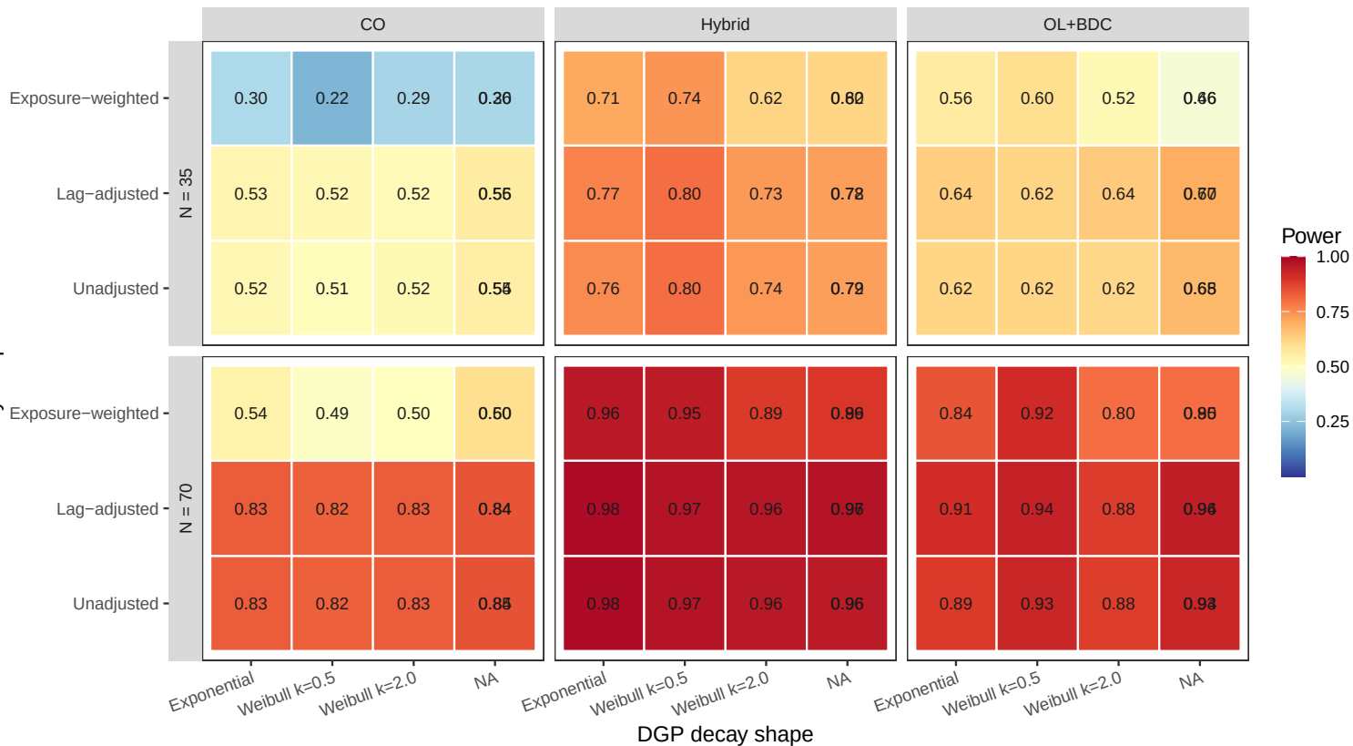
C (Architecture A): effect of DGP decay shape on power ( c_{bm} = 0.45 , t_{1/2} = 1 )
