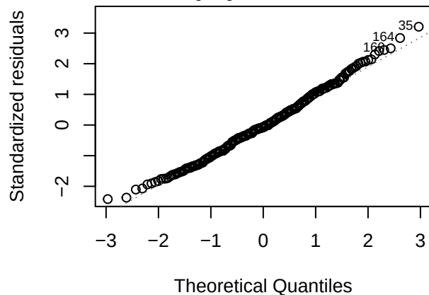
Q-Q Residuals
